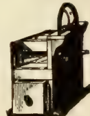
Box pattern; capacity, 15 lbs. an hour. Perforated tin cylinder, $8.50. Wooden cylinder, studded steel pins, $9.50.
